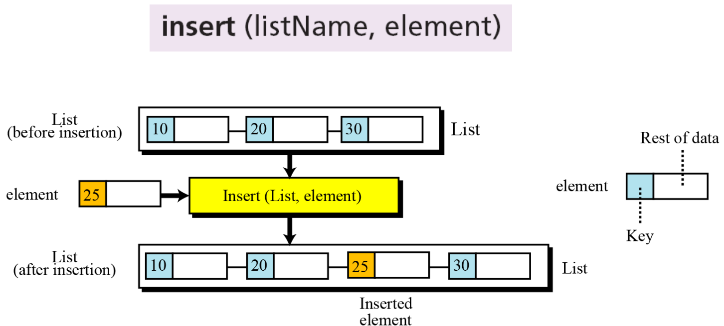
Figure 12.15 The insert operation
