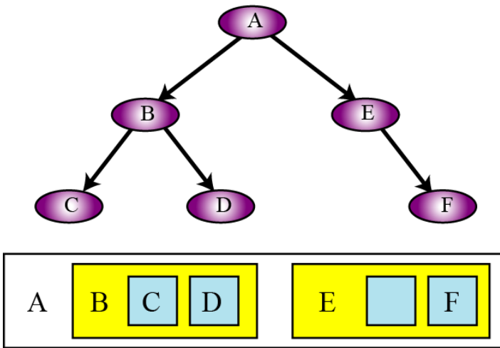
a. Processing order
