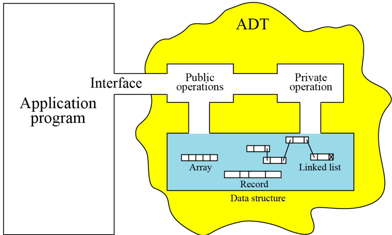
Figure 12.1 The model for an ADT
