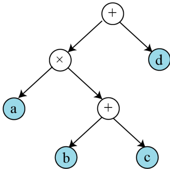
Expression tree
