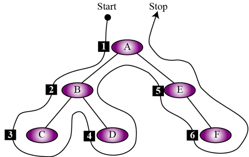
b. "Walking" order
